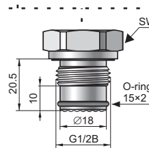
CG1/2 type G1/2" with flush diaphragm
