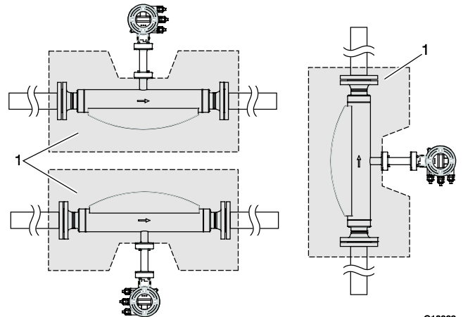
Fig. 10: Installation at T_{\text{medium}} -50^{\circ}\dots 200^{\circ}\text{C} (-58 ... 392 °F)
