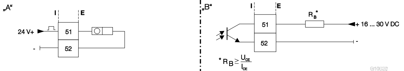
Fig. 28: Active / passive pulse output
