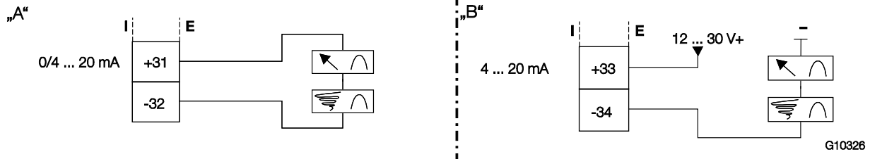
Fig. 26: Active / passive current outputs
