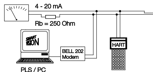
Fig. 24: Communication via HART protocol
